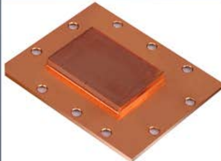
Copper base with micro channels
